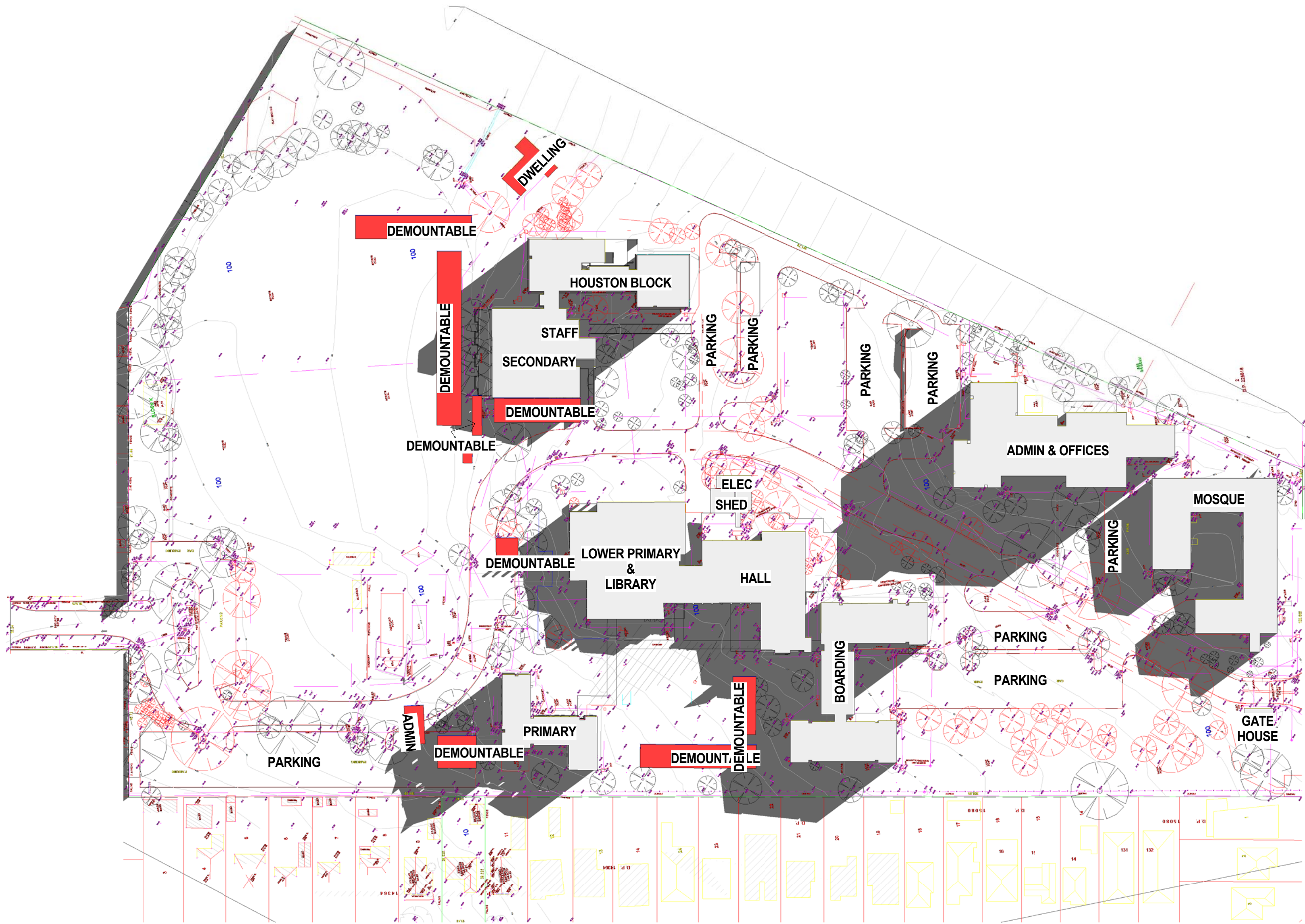
1 Existing - Shadow Diagram June 21 - 08am 1 : 1000
